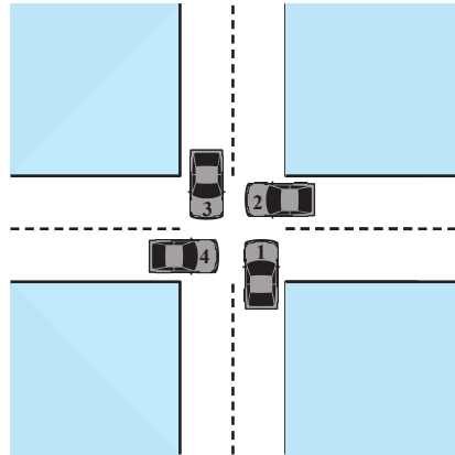
(b) Deadlock
